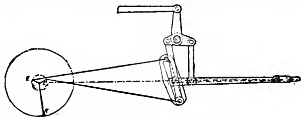
FIG. 31.—Allan's Link-Motion.
