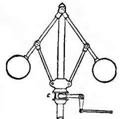
FIG. 42.—Watt's Governor.
