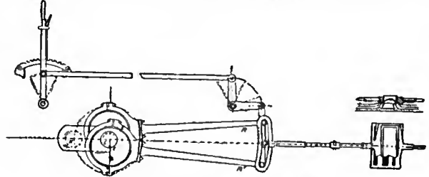
FIG. 29.—Stephenson's Link-Motion.
