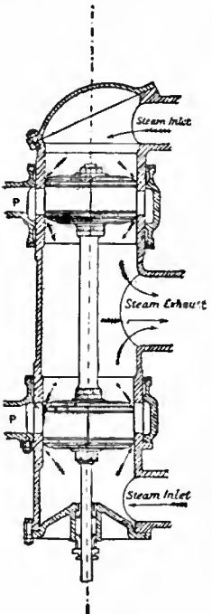
FIG. 40.—Piston Slide-Valve.
