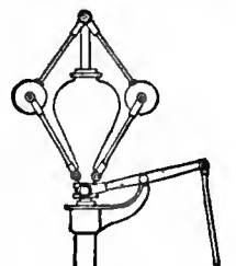
FIG. 43.—Loaded Governor.
