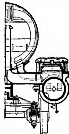
FIG. 51.—American Outside-Cylinder Locomotive.
