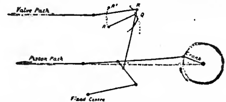
FIG. 35.—Diagram of Joy's Valve-Gear.
