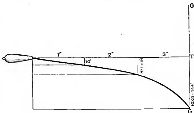
FIG. 1.—Elevation.
