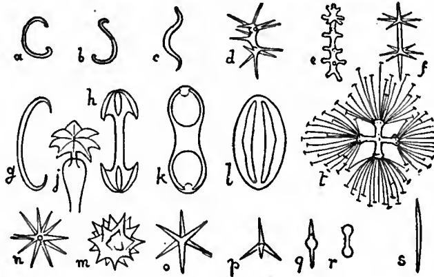
FIG. 30.—Typical Microscleres.
