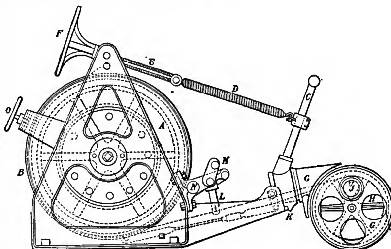
FIG. 1.—Lucas Machine.
