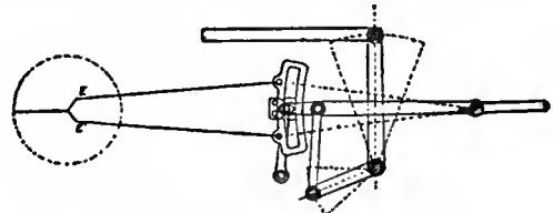
FIG. 30.—Gooch's Link-Motion.
