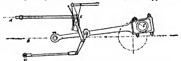
FIG. 36.—Joy's Gear as applied to a Locomotive.
