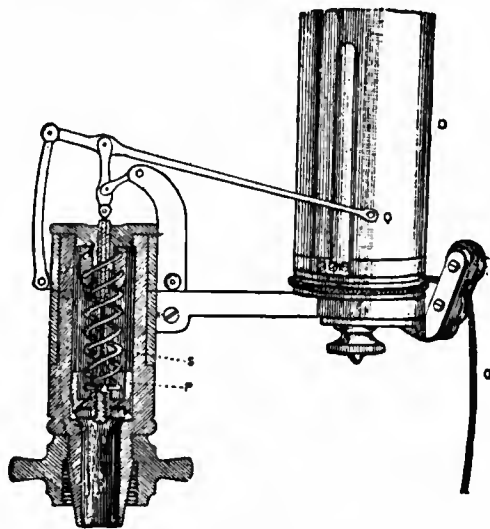
FIG. 15.—Crosby Indicator.
