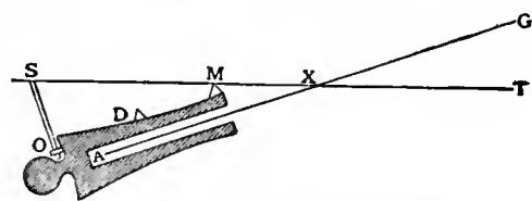
FIG. 4.—Theory of Tangent Sight.
