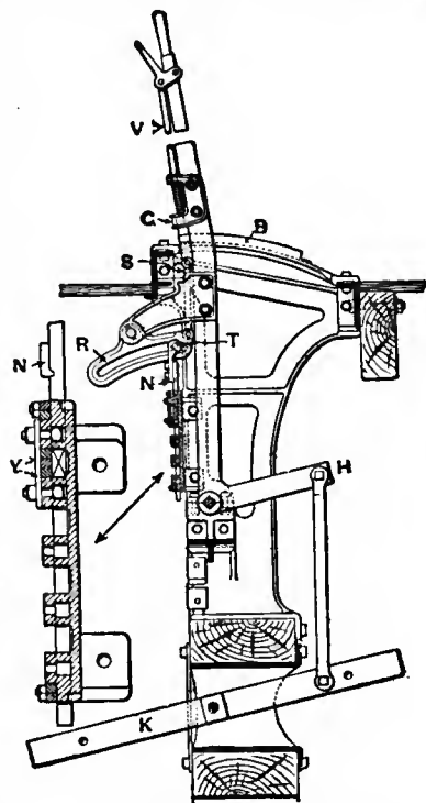
FIG. 6.—Signal Lever, with Mechanical Interlocking.
