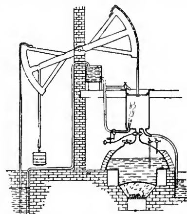
FIG. 4.—Newcomen's Atmospheric Engine, 1705.
