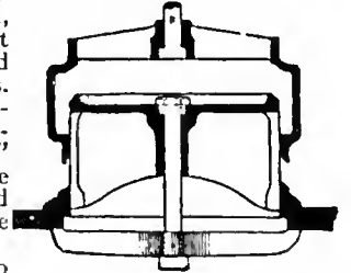
FIG. 41.—Double-Beat Lift Valve.
