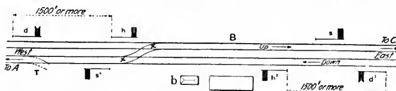
FIG. 8.—Block signals. (English practice, trains run on left-hand track, signals at left of track, arms on left of post.)
