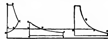
FIG. 16.—Compound Diagrams: Woolf type.
